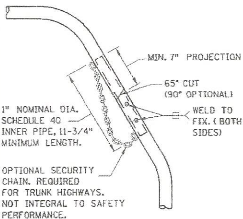
JOINT DETAIL
